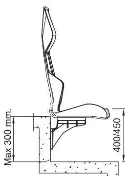
MENSOLA IN POLIAMMIDE POLYAMIDE BRACKET
