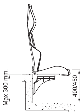
MENSOLA IN POLIAMMIDE POLYAMIDE BRACKET
