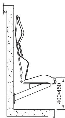
MENSOLA IN MMETALLO METAL BRACKET
