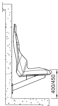
MENSOLA IN METALLO METAL BRACKET
