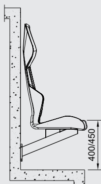
MENSOLA IN MMETALLO METAL BRACKET
